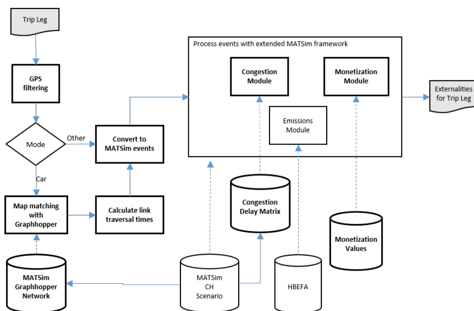
Figure 6 – MATSim-based externalities pipeline
